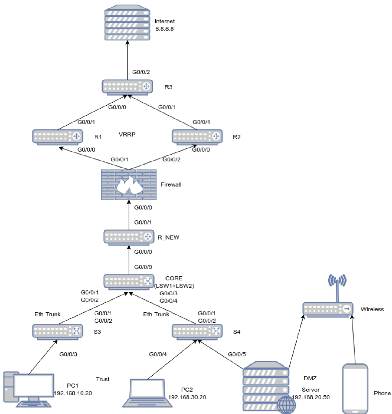
Figure 1: 实验拓扑图
