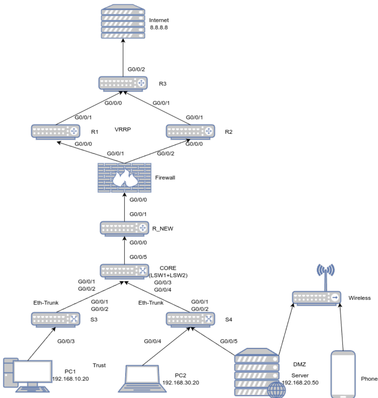
Figure 1: 实验拓扑图
