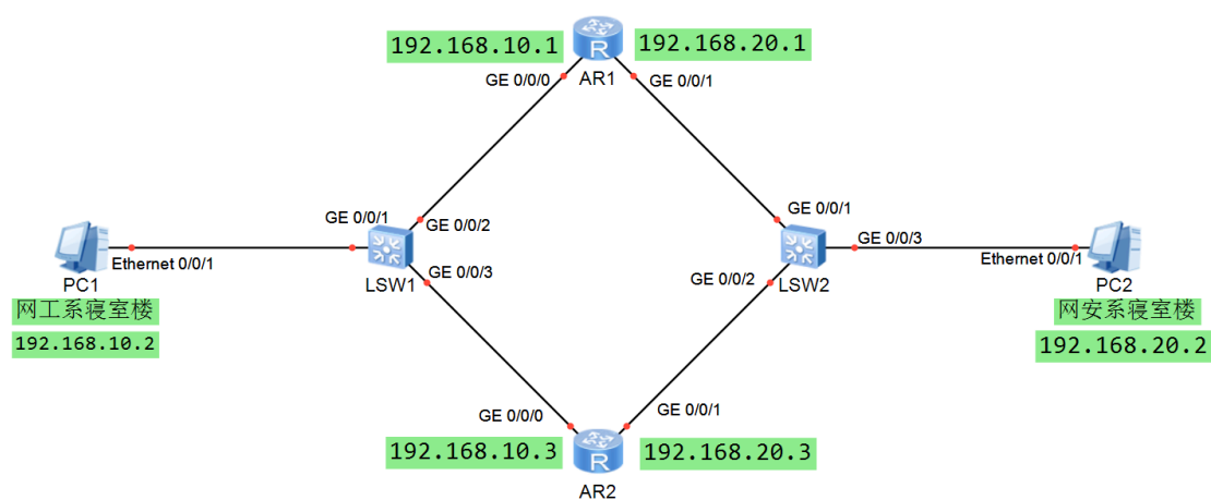
Figure 1: 实验拓扑图
