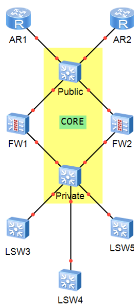
Figure 2: 逻辑拓扑图
