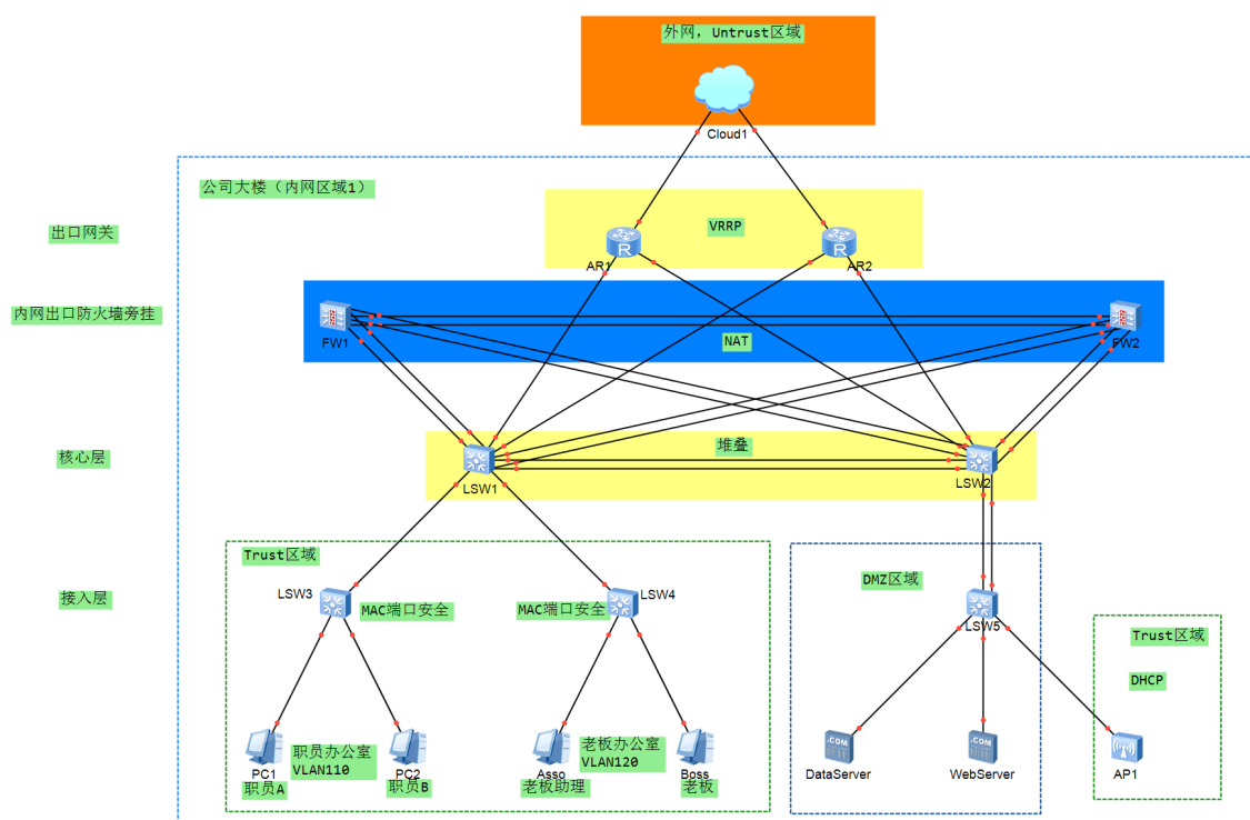
Figure 1: 实验拓扑图
