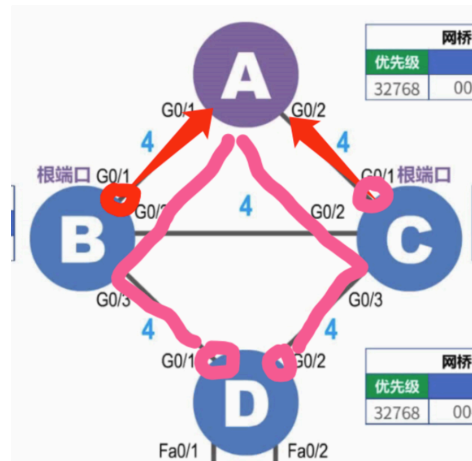
Figure 2: 链路成本示例
