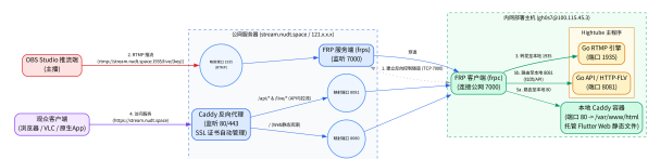
Figure 3: Hightube 系统网络部署拓扑结构图
